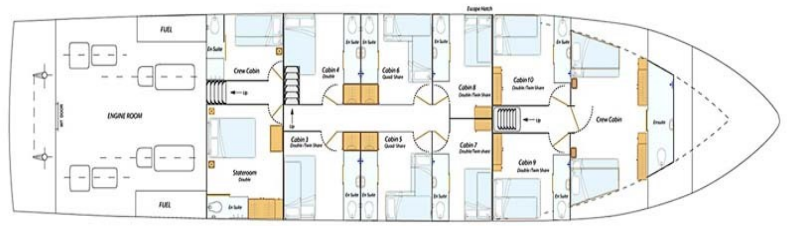
Below Deck Layout & Accommodation
